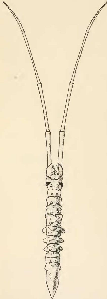
FIG. 24.—ARCTURUS HASTIGER. \times 1\frac{1}{2} . (Drawn by Miss V. Dandridge.)
